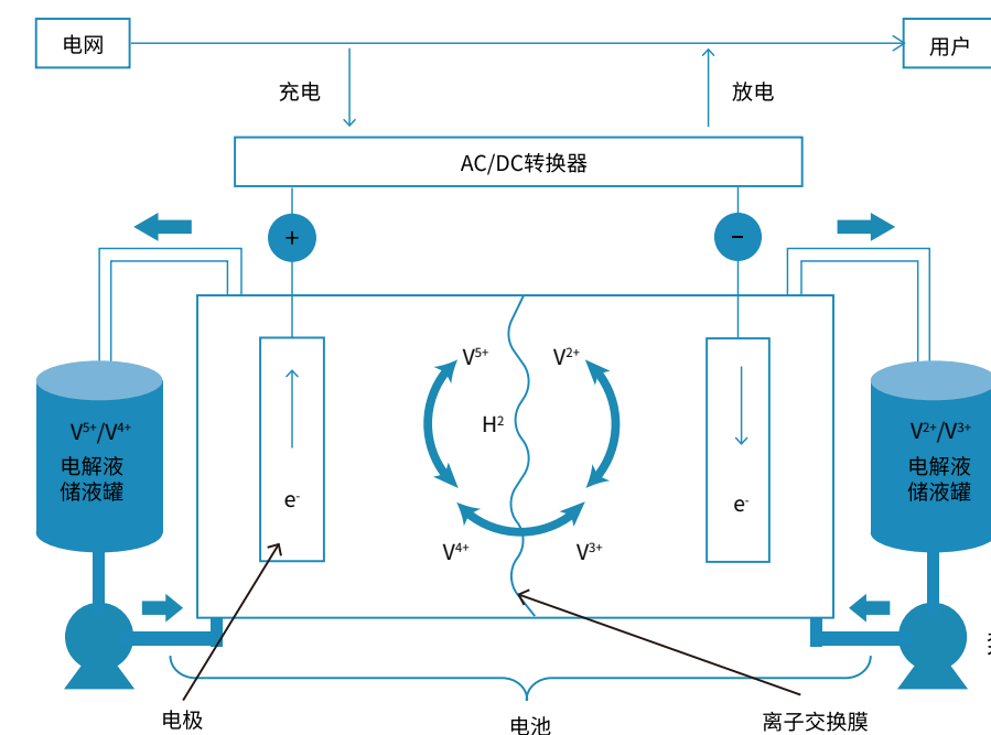
液流电池储能流程示意图 Schematic diagram of flow battery energy storage process
